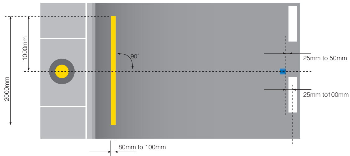
BELOW GROUND, OFF ROAD, FIRE HYDRANT - ROAD MARKINGS & REFLECTOR LOCATION
