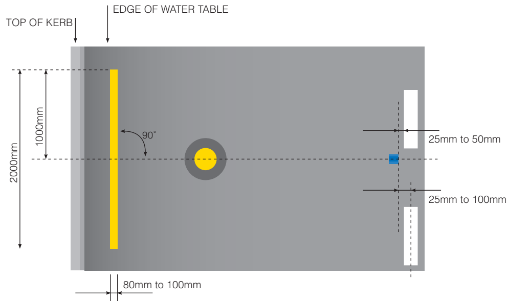
BELOW GROUND FIRE HYDRANT - ROAD MARKINGS & REFLECTOR LOCATION
