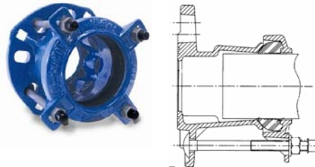
Adaptor Flange
