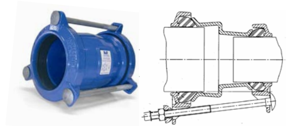
Stepped Coupling
