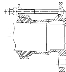
Adaptor Flange
